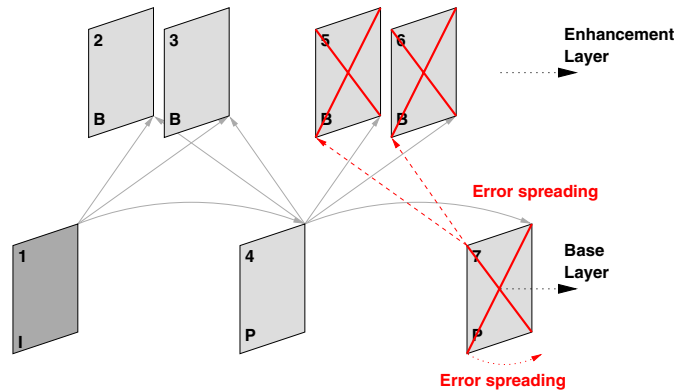
Fig. 1. Temporal scalable video with inter-frame dependencies and different error spreading possibilities.
