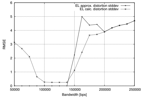
Fig. 4. Standard deviation of the distortion from approximation and calculation for spatial scalable video streaming of the News video sequence.
