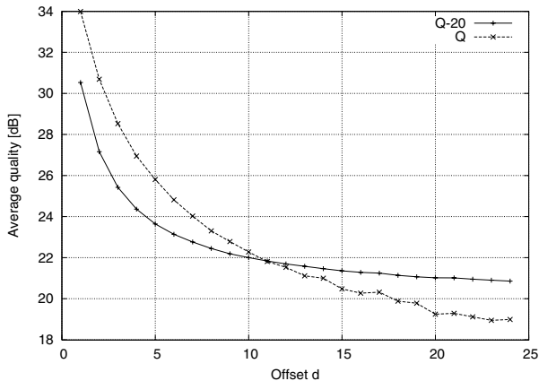
Fig. 8. Comparison of approximation of quality of loss-affected frames (Q-20) with actual quality obtained from offset distortion trace (Q): Average video stream qualities for the Foreman video sequence encoded with quantization scale q = 3 at different offsets for bit error rate 10^{-4} .
