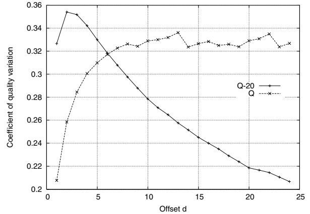
Fig. 9. Comparison of approximation of quality of loss-affected frames (Q-20) with actual quality obtained from offset distortion trace (Q): Coefficient of video frame quality variation for the Foreman video sequence encoded with quantization scale q = 3 at different offsets for bit error rate 10^{-4} .
