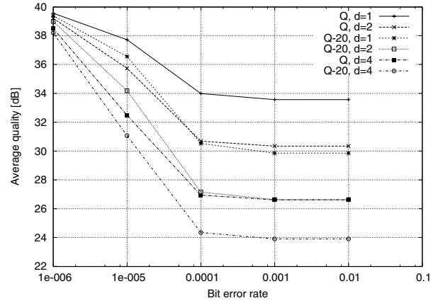
Fig. 6. Comparison of approximation of quality of loss-affected frames (Q-20) with actual quality obtained from offset distortion trace (Q): Average video qualities for the Foreman video sequence encoded with quantization scale q = 3 as function of bit error rate for different offsets d .
