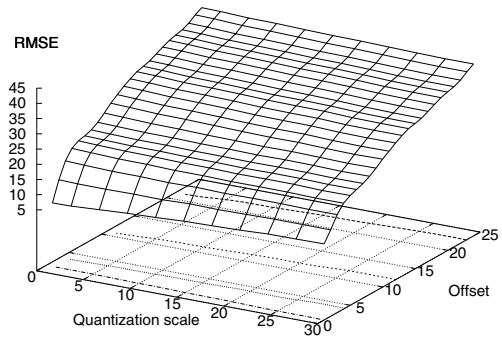
Fig. 10. Video frame offset distortion as function of the quantization scale and offset for frame 100 of the Foreman video sequence.
