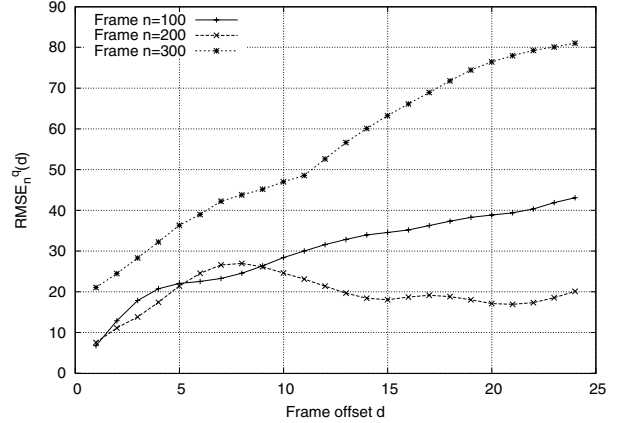
Fig. 3. Video frame offset distortion for frames n = 100, 200, and 300 from the Foreman video sequence encoded with quantization scale q = 3 .
