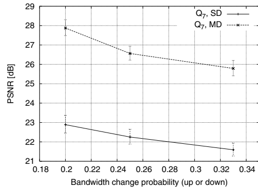
Fig. 5. Transmission quality for The Transporter base layer (QP=7) with different node mobilities modeled by the bandwidth change probability.
